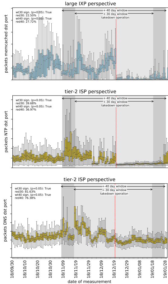
Figure 4: Selected significant changes in traffic before and after the takedown; wt_{30}/wt_{40} : significant lower packet counts at p = 0.05 when comparing 30/40 days before and after the takedown; red_{30}/red_{40} : ratio of daily mean 30/40 days before and 30/40 days after the takedown.
