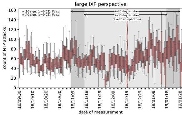
Figure 5: Systems under NTP DDoS attack per hour.
